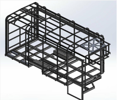
Galvanized Steel Cage Structure
